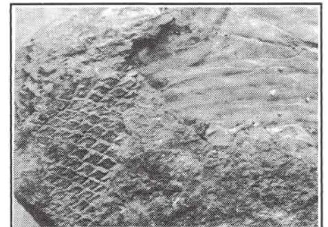
New strata on old.
