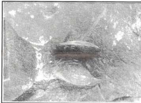
Fossil fresh water mussel
